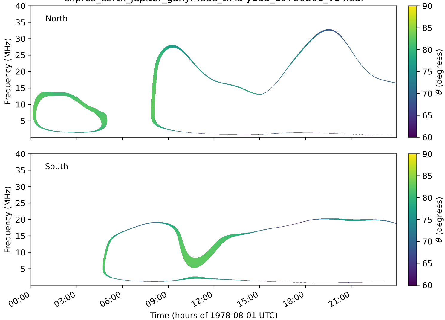
expres_earth_jupiter_ganymede_txka-y235_19780801_v14.cdf
