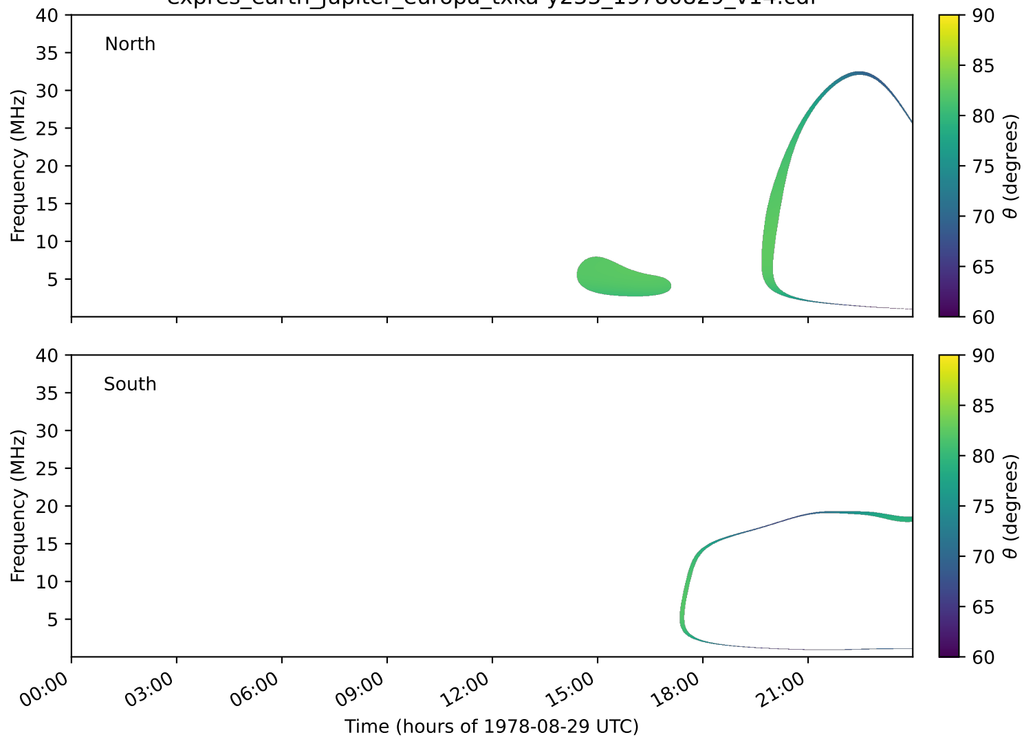
expres_earth_jupiter_europa_txka-y235_19780829_v14.cdf
