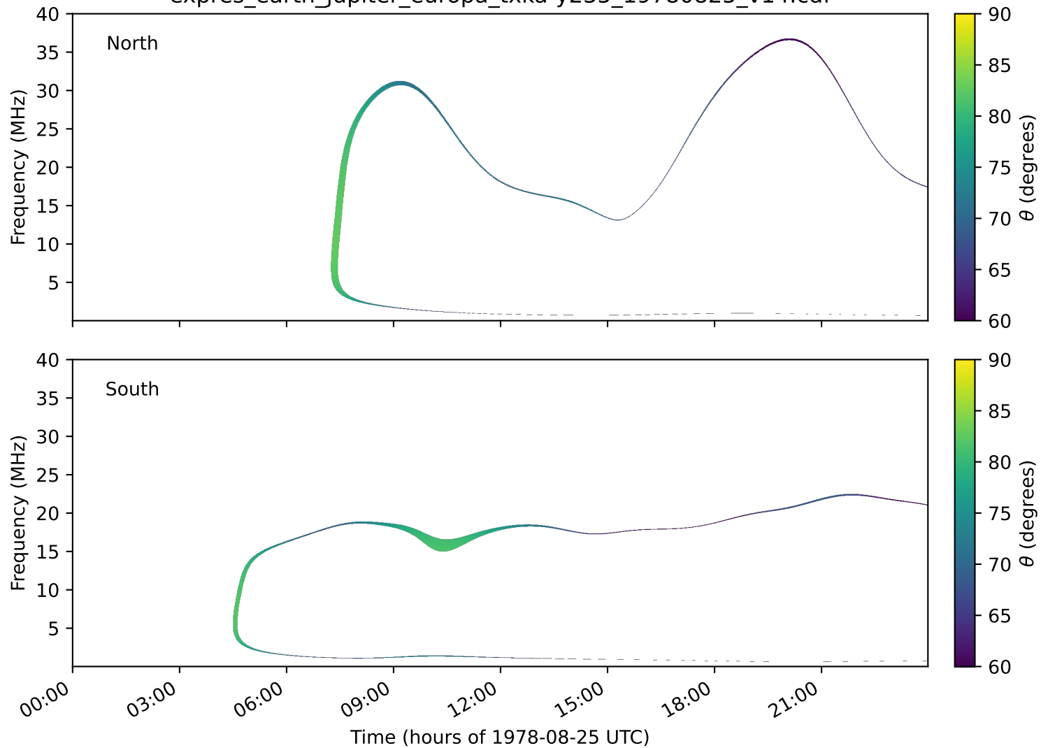
expres_earth_jupiter_europa_txka-y235_19780825_v14.cdf
