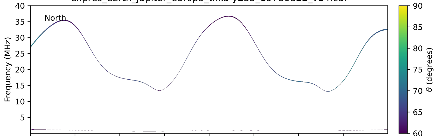
expres_earth_jupiter_europa_txka-y235_19780822_v14.cdf
