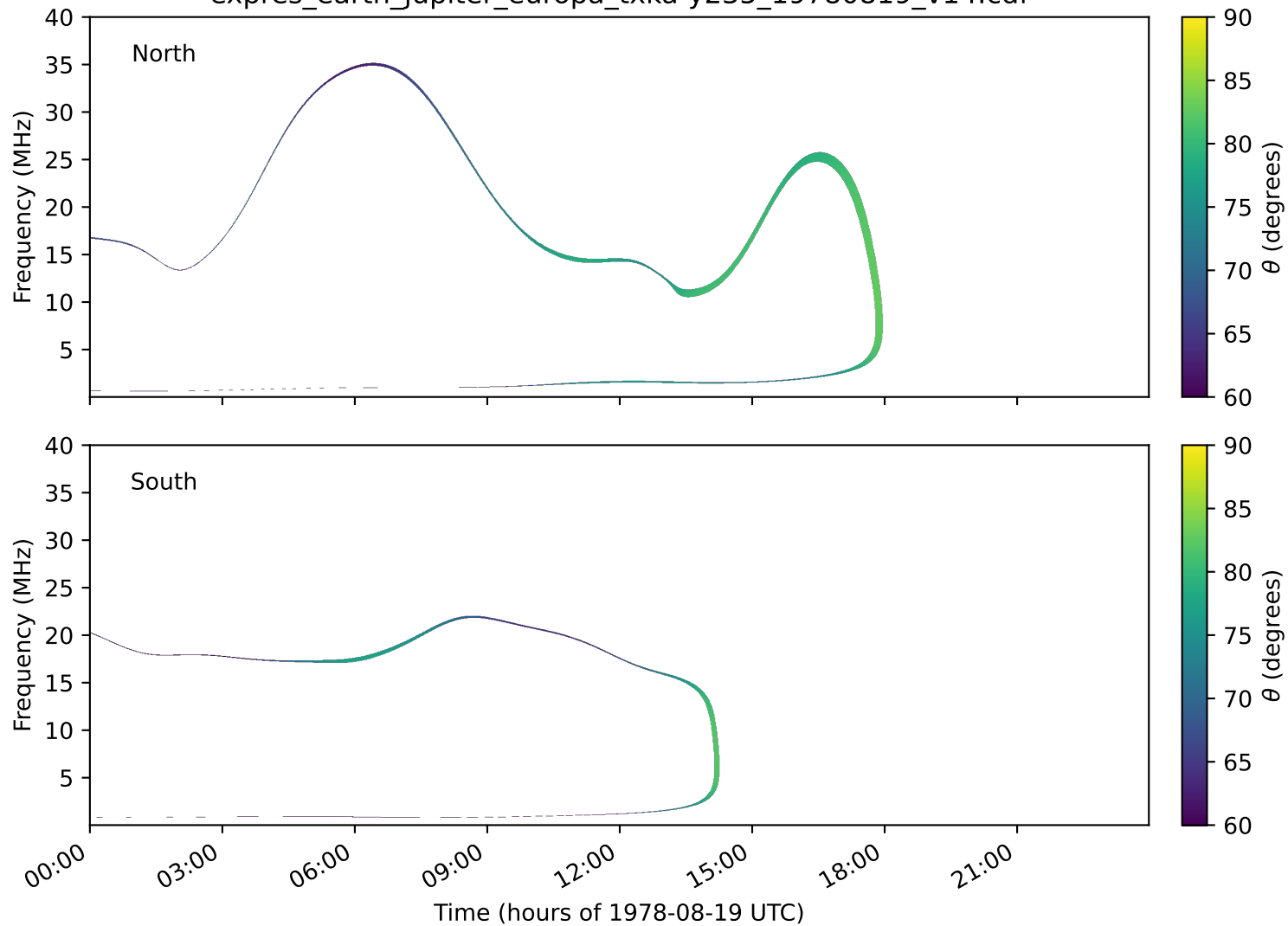
expres_earth_jupiter_europa_txka-y235_19780819_v14.cdf
