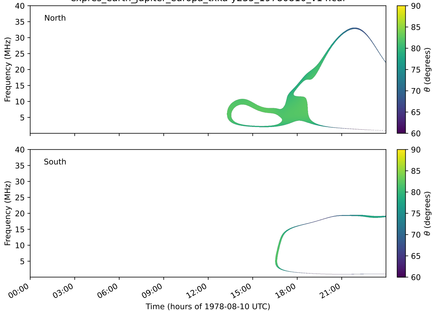
expres_earth_jupiter_europa_txka-y235_19780810_v14.cdf
