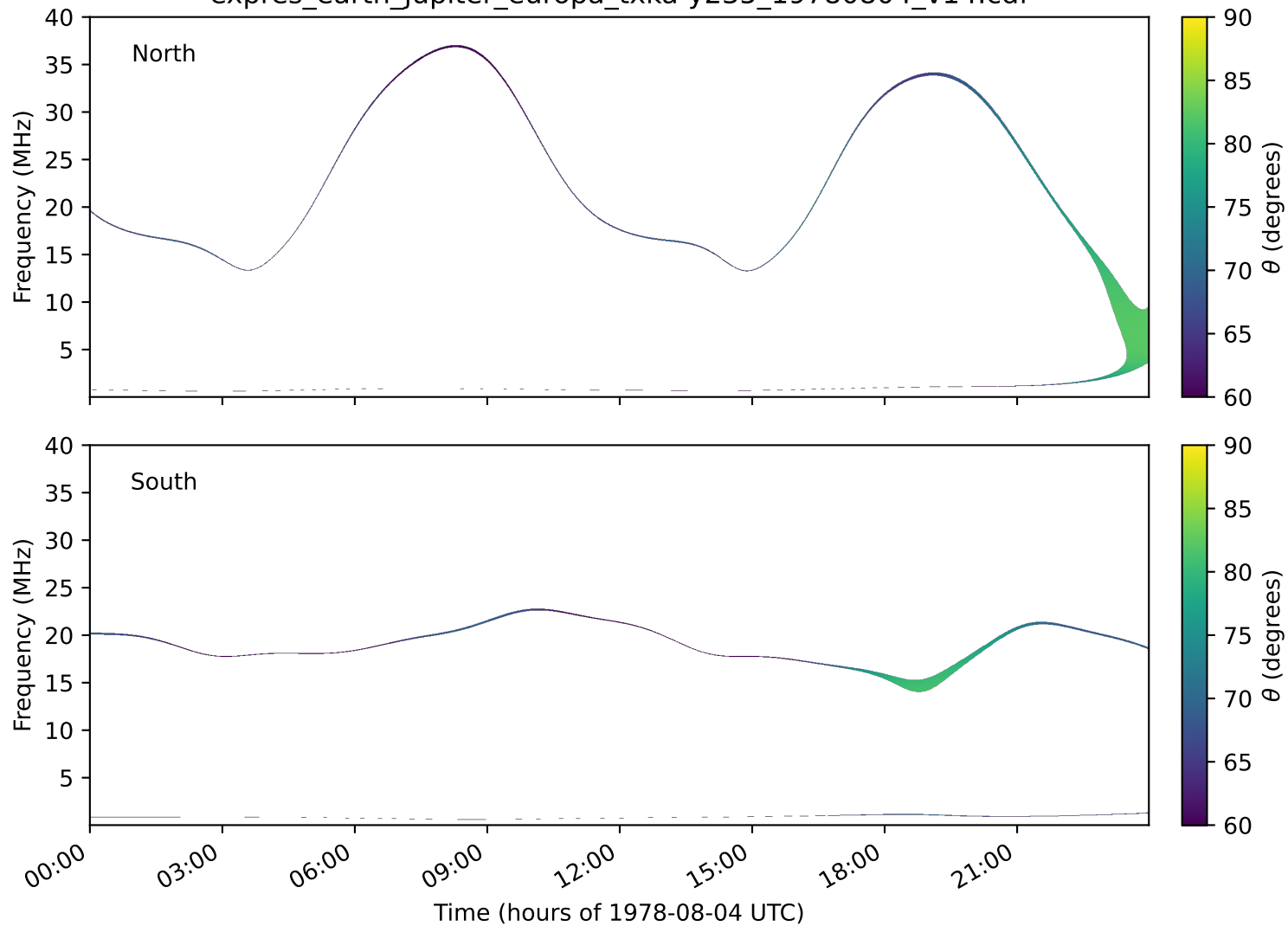
expres_earth_jupiter_europa_txka-y235_19780804_v14.cdf
