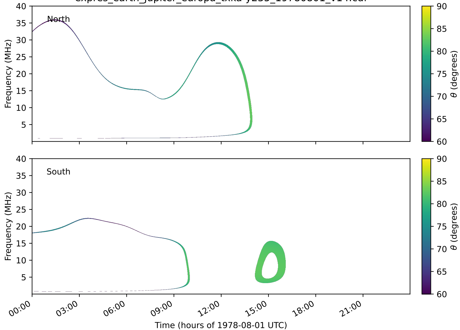
expres_earth_jupiter_europa_txka-y235_19780801_v14.cdf
