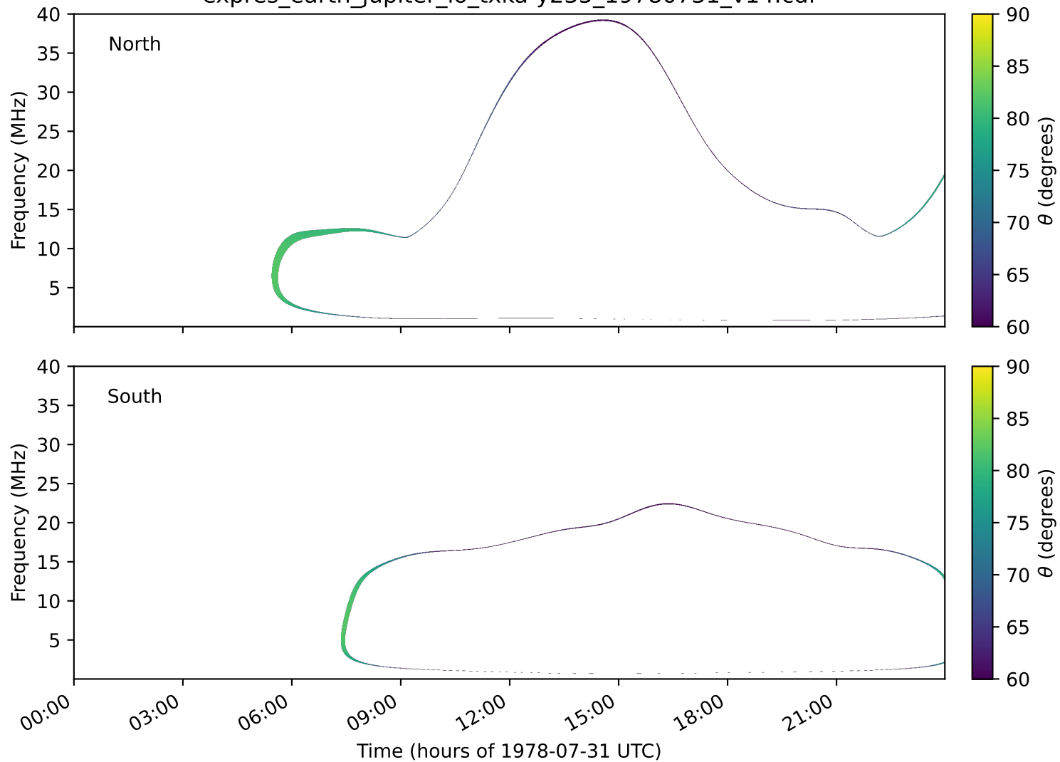
expres_earth_jupiter_io_txka-y235_19780731_v14.cdf
