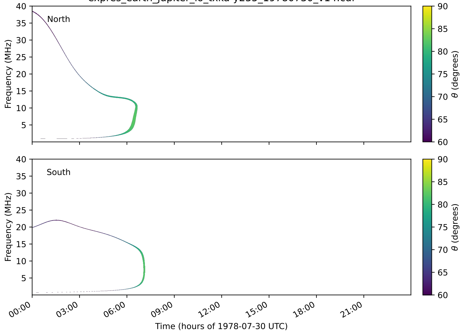
expres_earth_jupiter_io_txka-y235_19780730_v14.cdf
