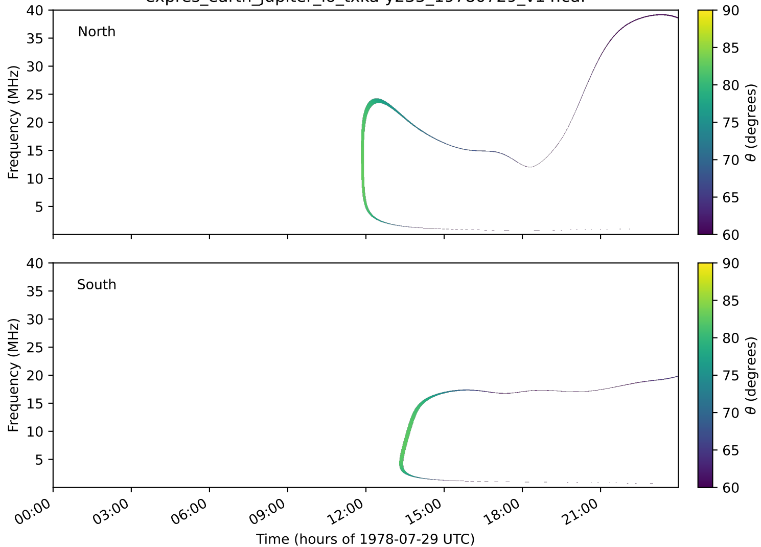
expres_earth_jupiter_io_txka-y235_19780729_v14.cdf
