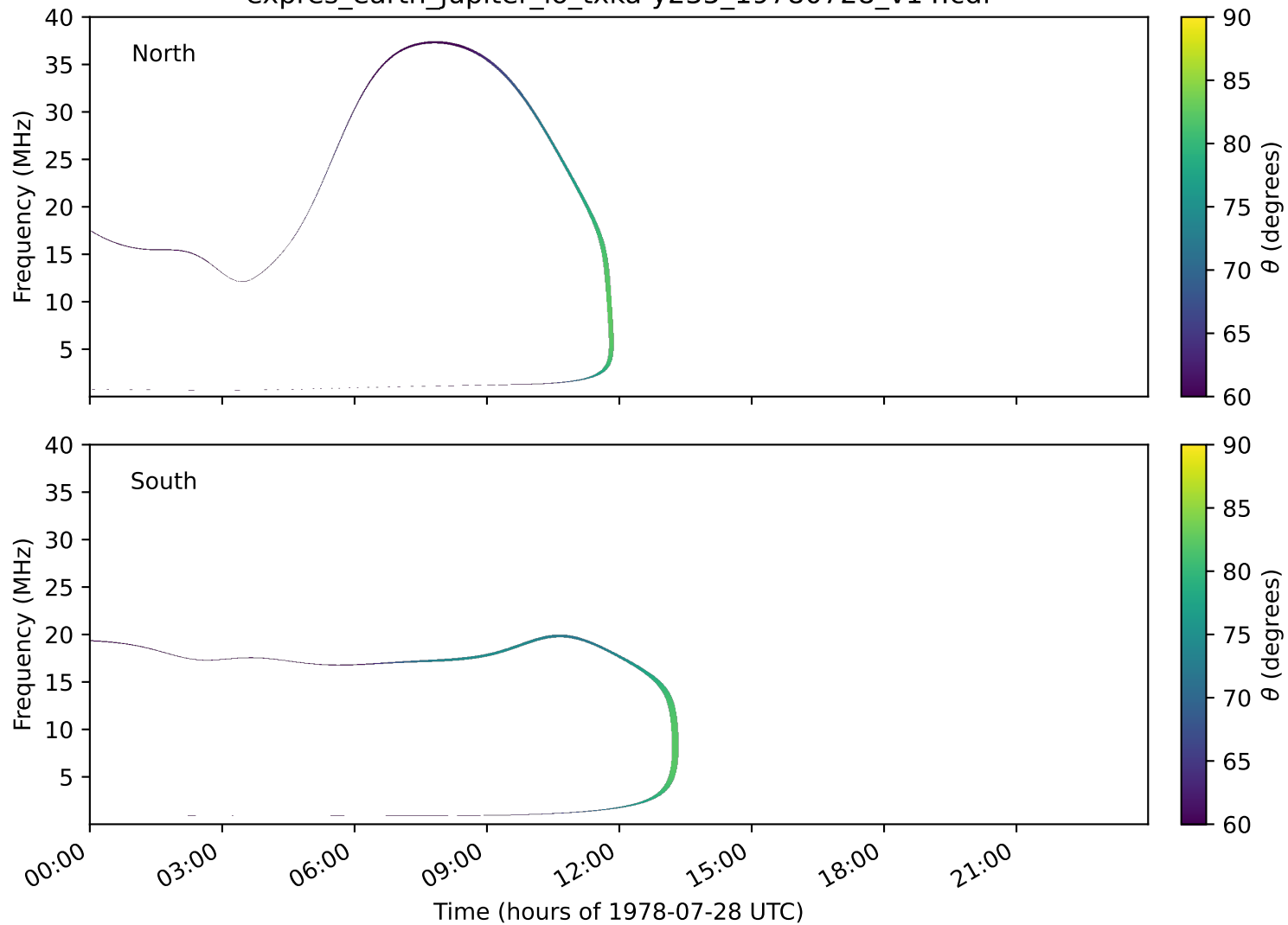
expres_earth_jupiter_io_txka-y235_19780728_v14.cdf
