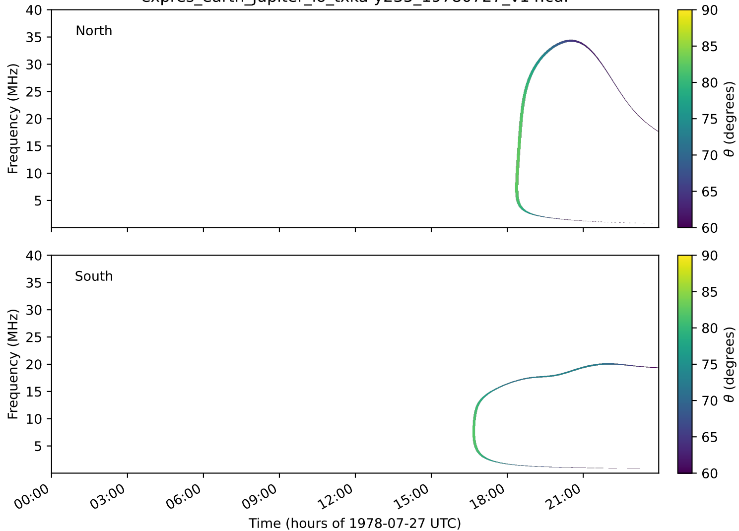
expres_earth_jupiter_io_txka-y235_19780727_v14.cdf
