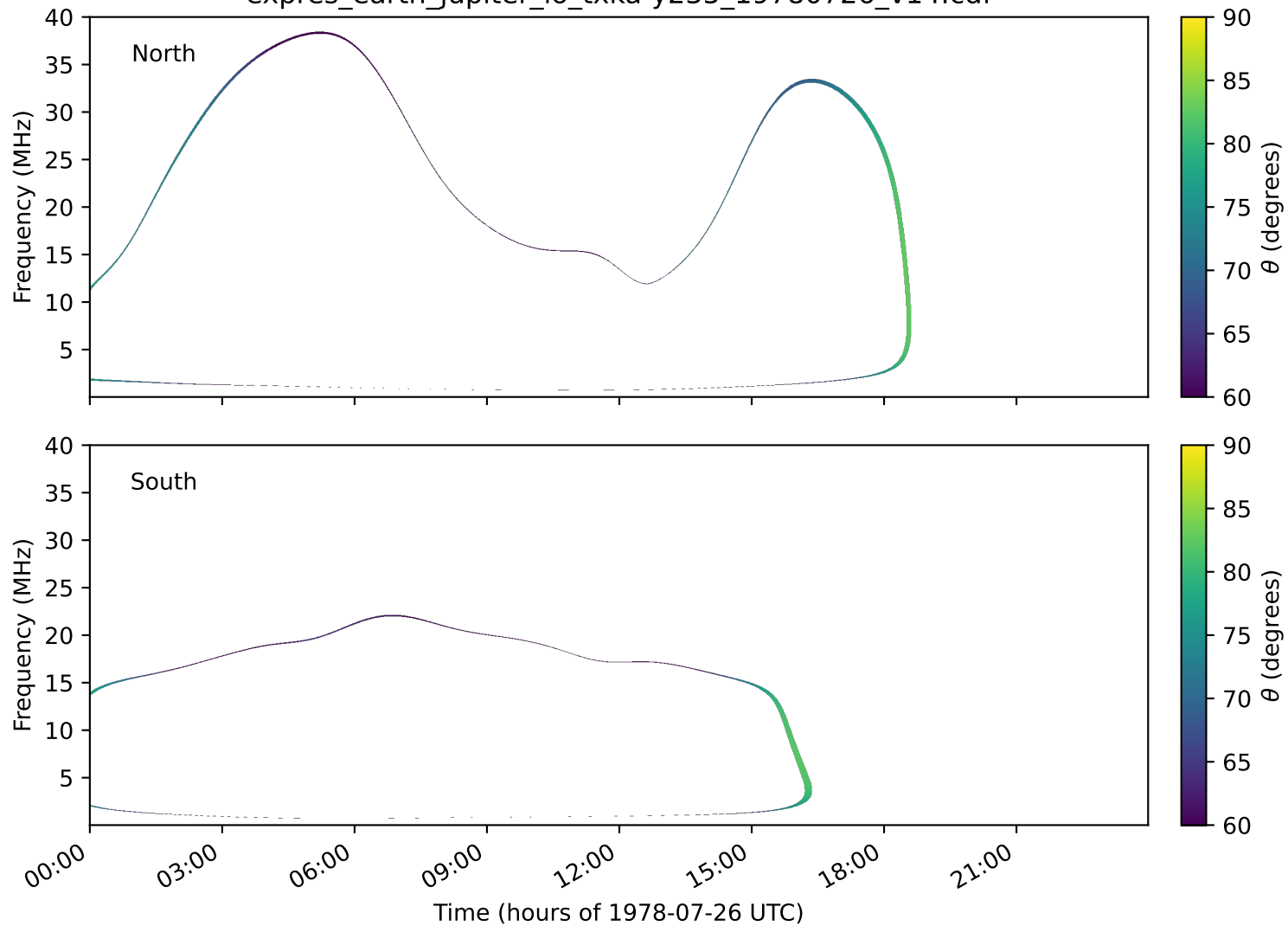
expres_earth_jupiter_io_txka-y235_19780726_v14.cdf
