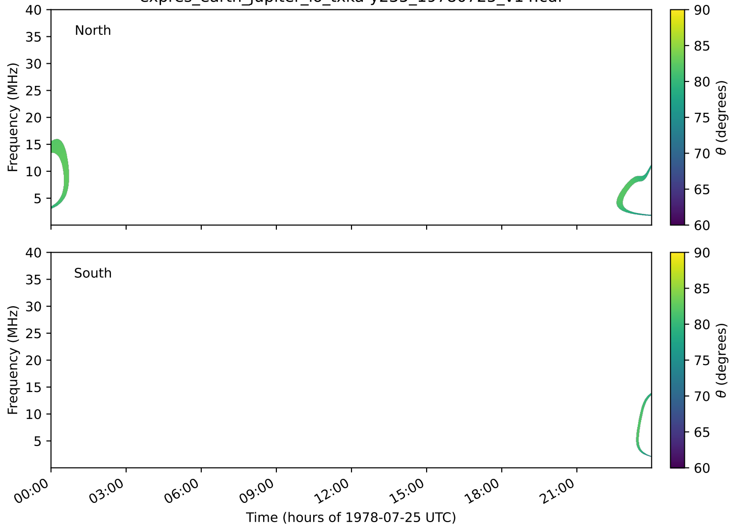
expres_earth_jupiter_io_txka-y235_19780725_v14.cdf
