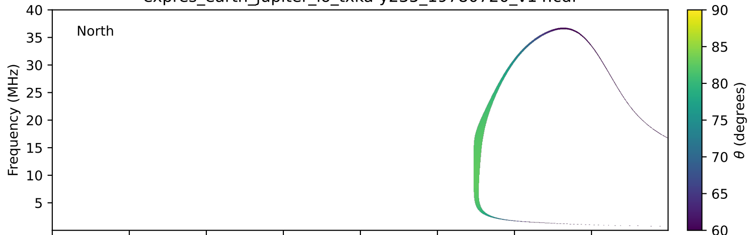
expres_earth_jupiter_io_txka-y235_19780720_v14.cdf
