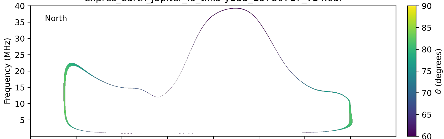
expres_earth_jupiter_io_txka-y235_19780717_v14.cdf
