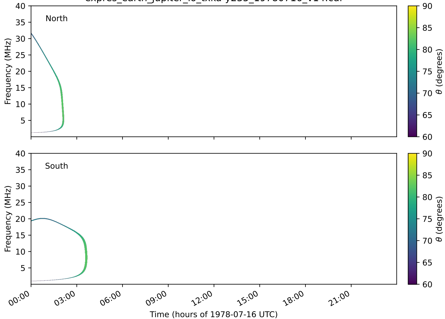
expres_earth_jupiter_io_txka-y235_19780716_v14.cdf
