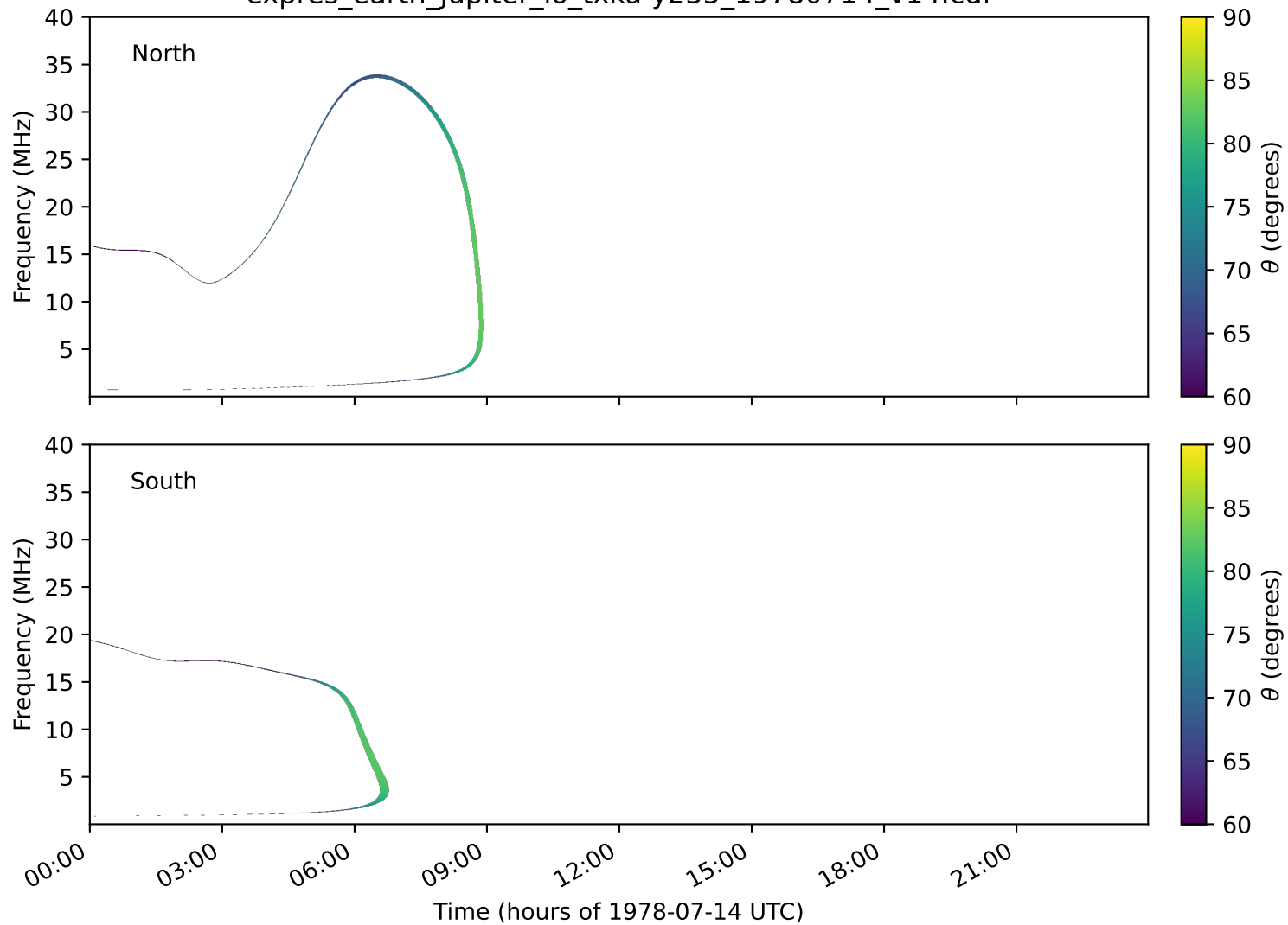
expres_earth_jupiter_io_txka-y235_19780714_v14.cdf
