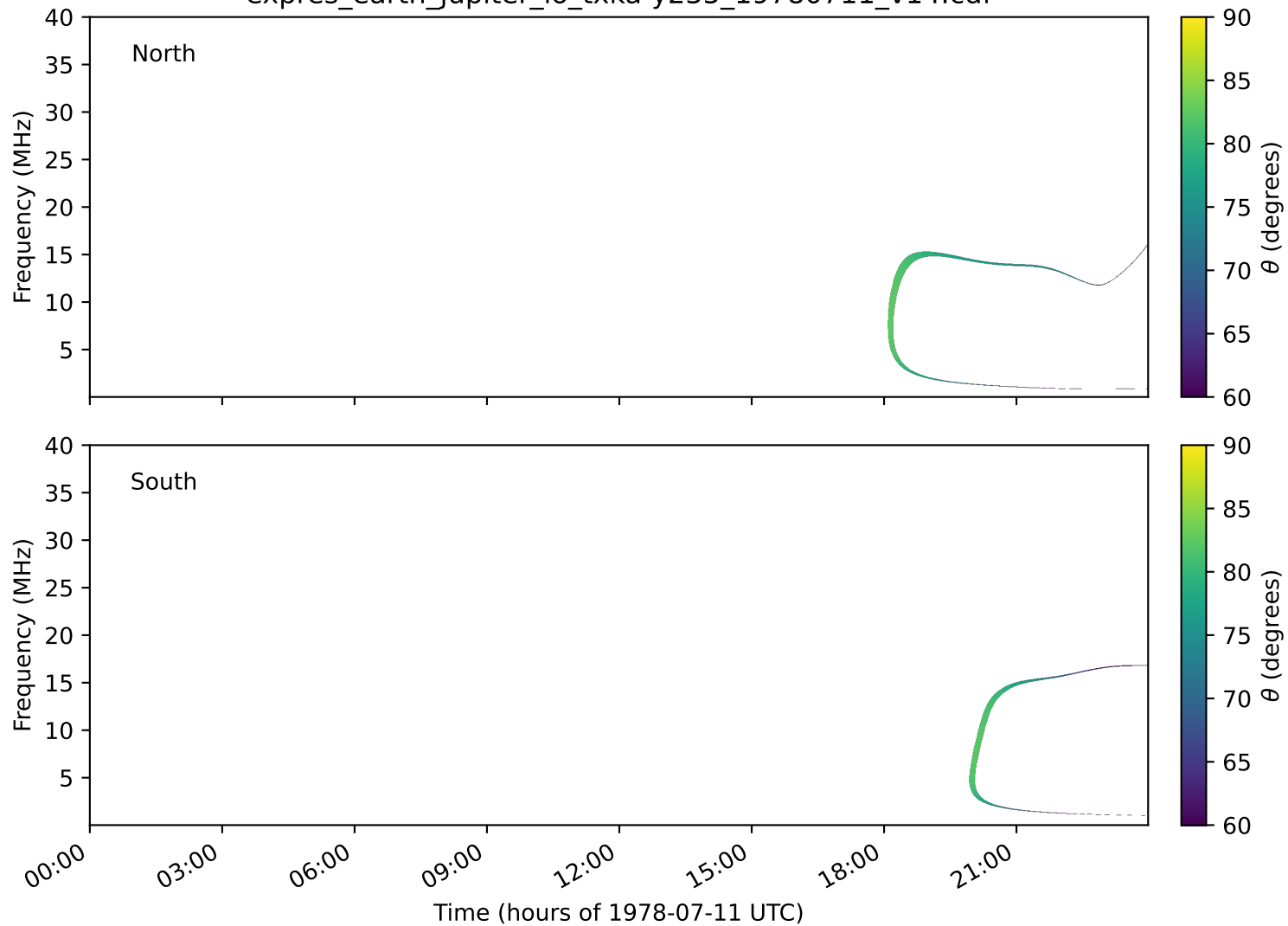
expres_earth_jupiter_io_txka-y235_19780711_v14.cdf
