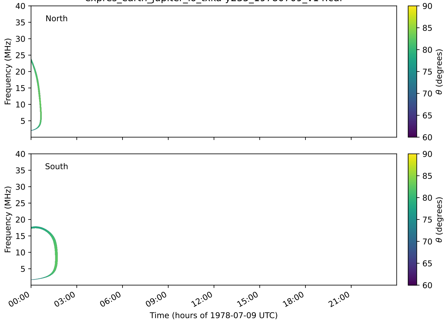
expres_earth_jupiter_io_txka-y235_19780709_v14.cdf
