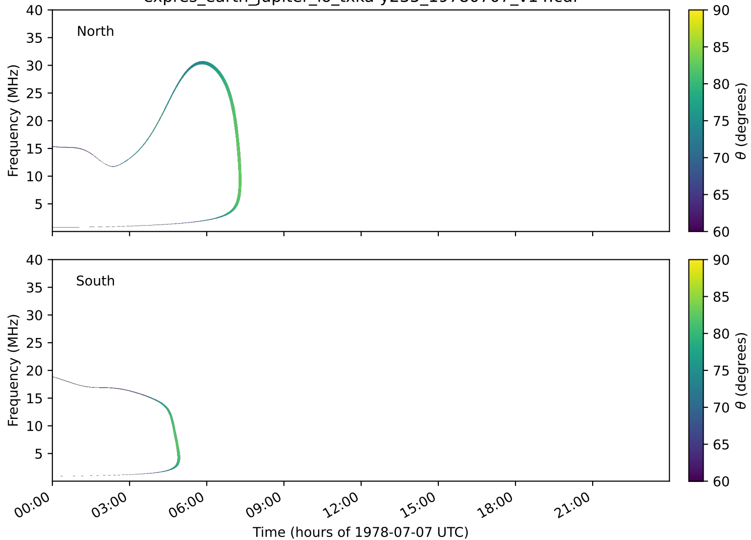
expres_earth_jupiter_io_txka-y235_19780707_v14.cdf
