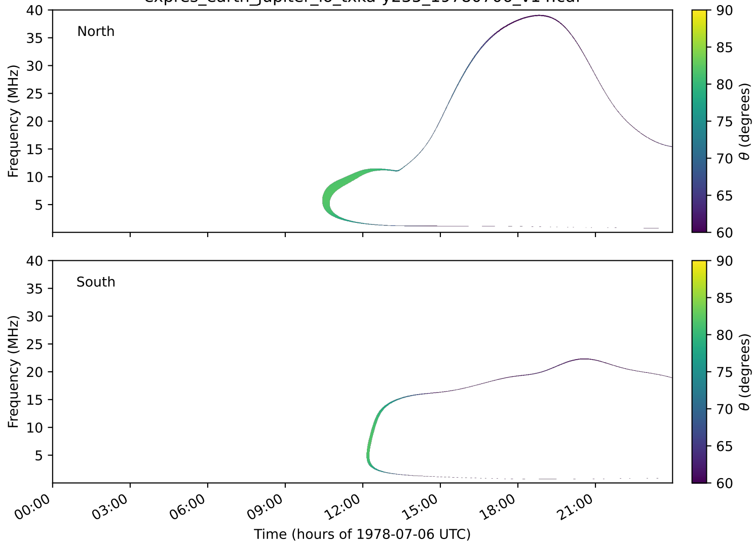
expres_earth_jupiter_io_txka-y235_19780706_v14.cdf
