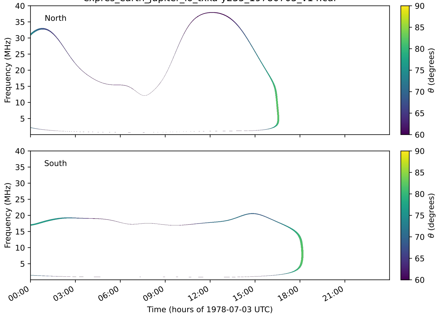
expres_earth_jupiter_io_txka-y235_19780703_v14.cdf
