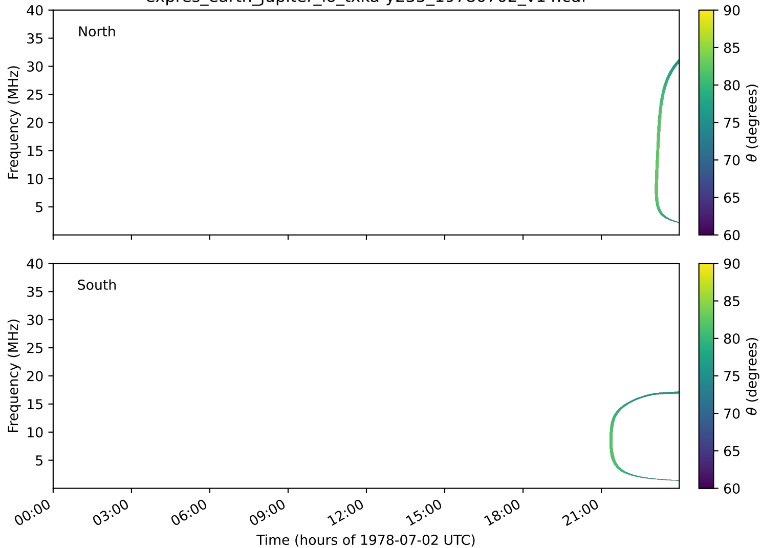
expres_earth_jupiter_io_txka-y235_19780702_v14.cdf
