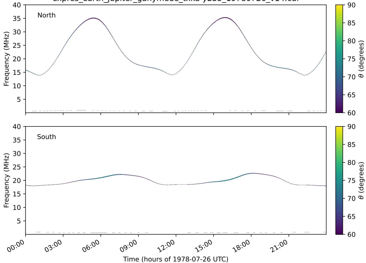
expres_earth_jupiter_ganymede_txka-y235_19780726_v14.cdf
