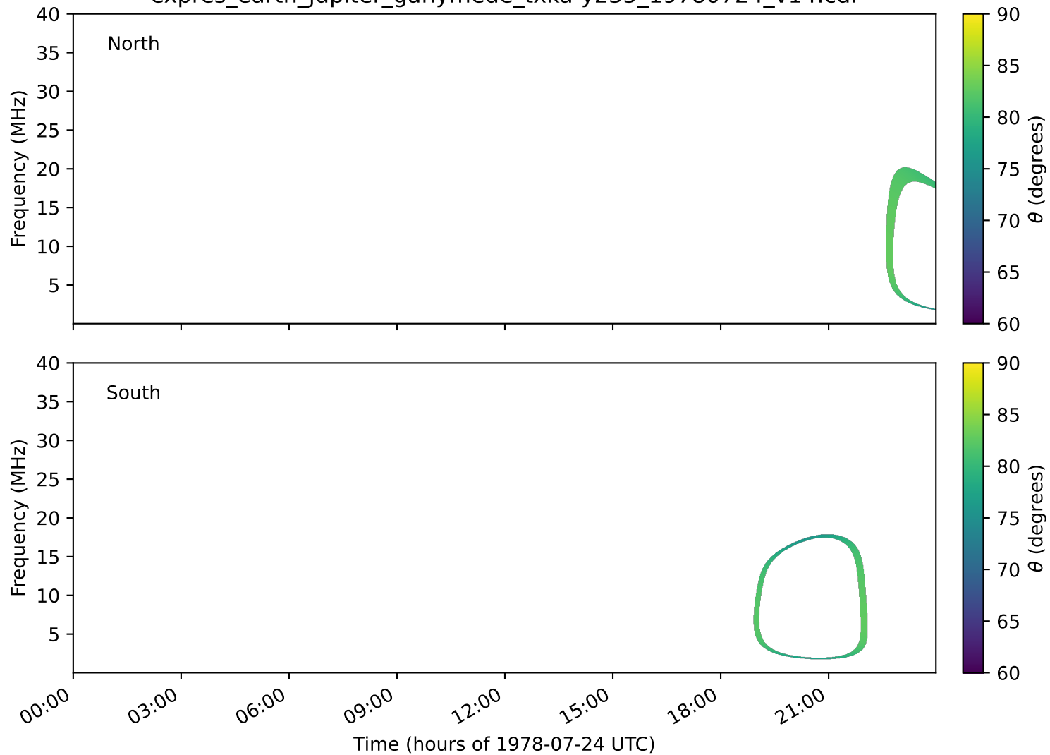
expres_earth_jupiter_ganymede_txka-y235_19780724_v14.cdf
