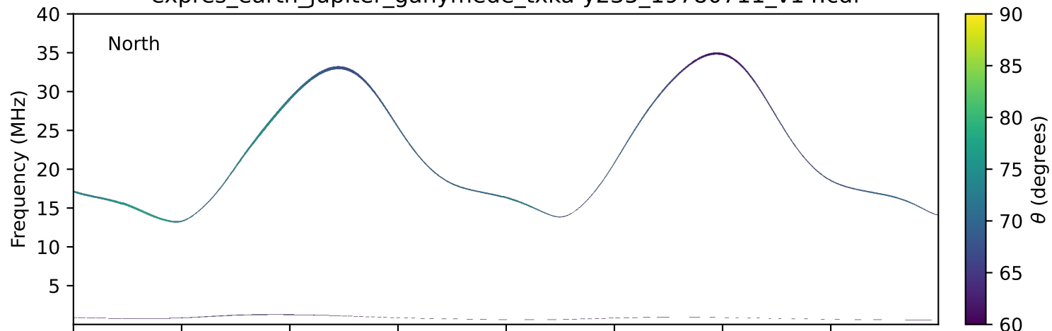
expres_earth_jupiter_ganymede_txka-y235_19780711_v14.cdf
