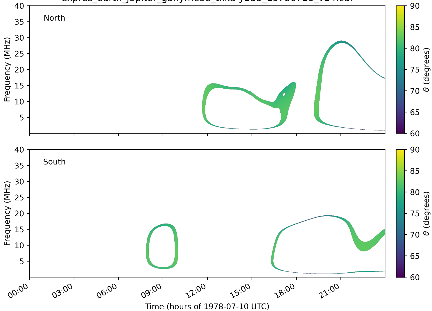
expres_earth_jupiter_ganymede_txka-y235_19780710_v14.cdf
