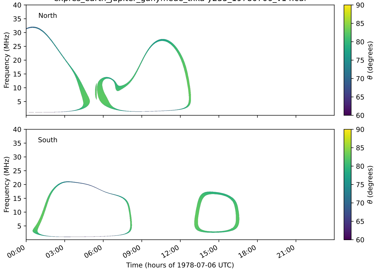
expres_earth_jupiter_ganymede_txka-y235_19780706_v14.cdf
