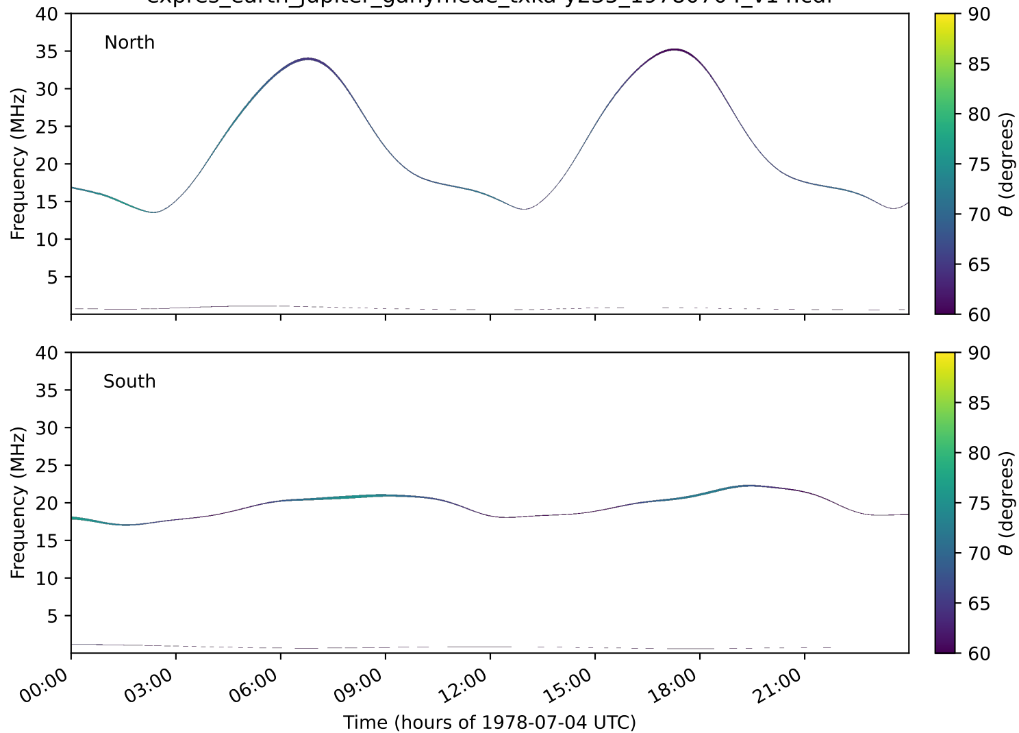
expres_earth_jupiter_ganymede_txka-y235_19780704_v14.cdf
