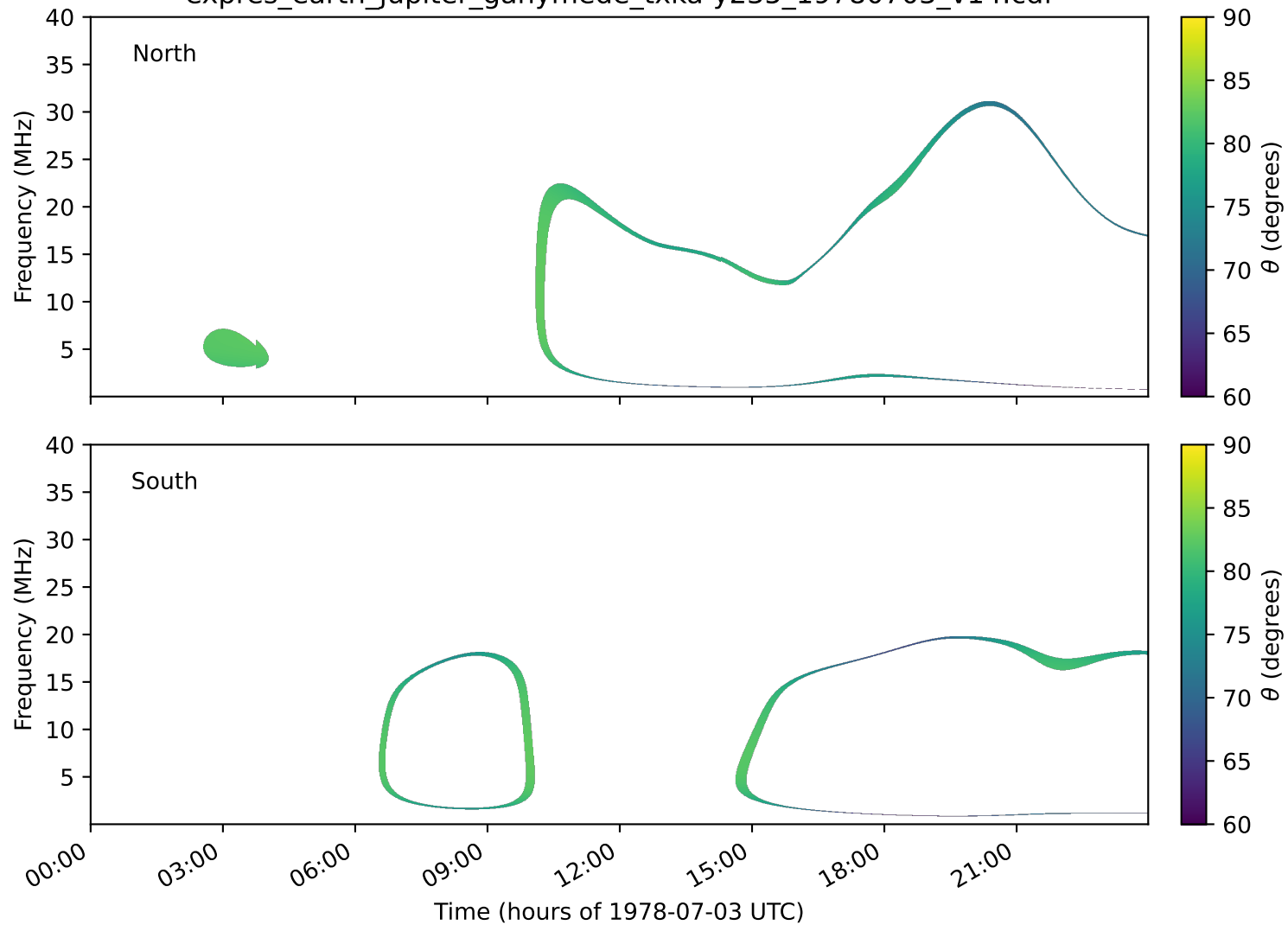
expres_earth_jupiter_ganymede_txka-y235_19780703_v14.cdf
