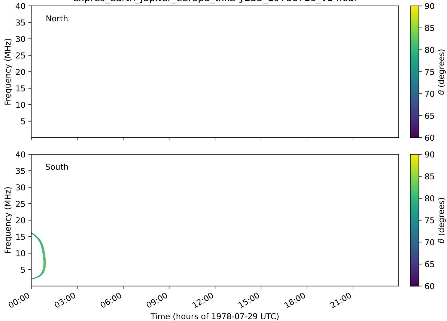
expres_earth_jupiter_europa_txka-y235_19780729_v14.cdf
