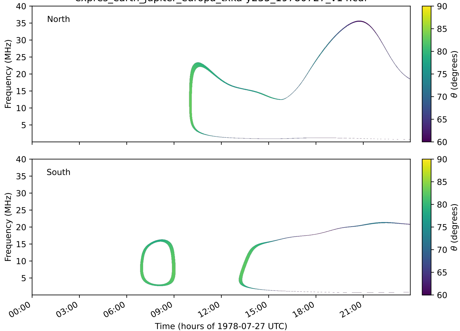
expres_earth_jupiter_europa_txka-y235_19780727_v14.cdf
