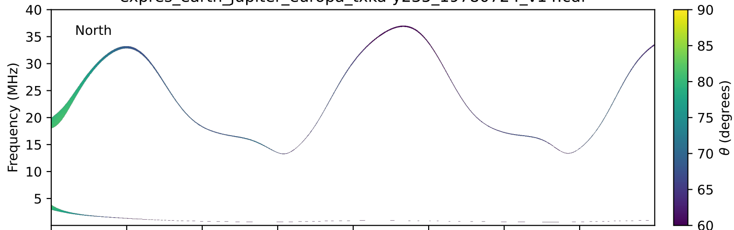
expres_earth_jupiter_europa_txka-y235_19780724_v14.cdf
