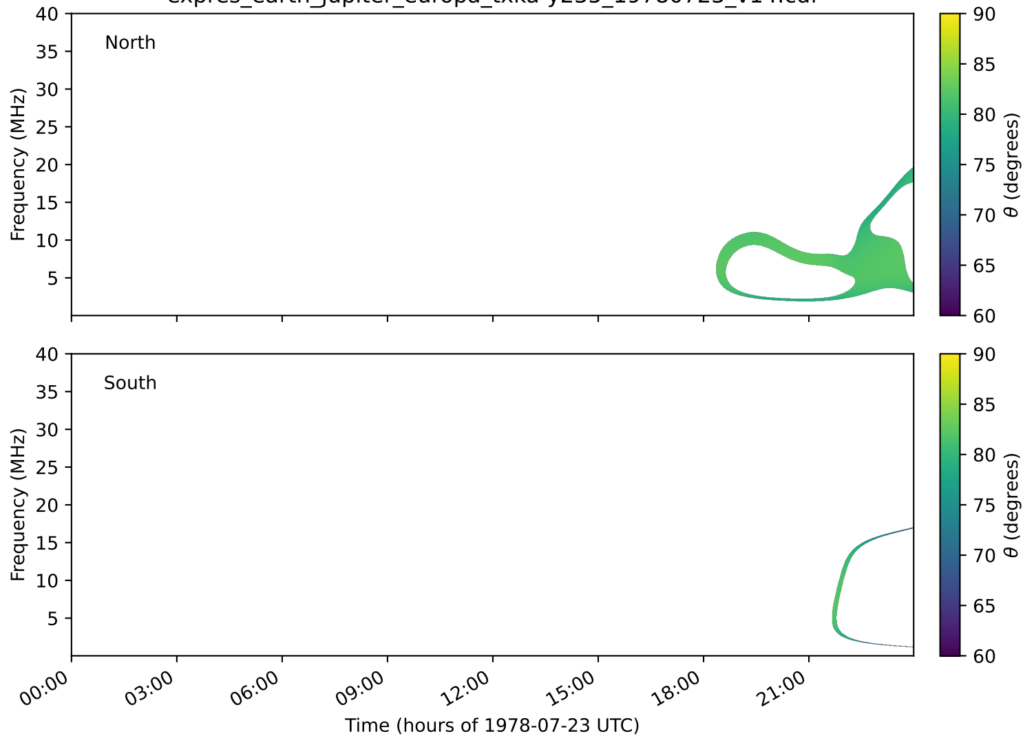
expres_earth_jupiter_europa_txka-y235_19780723_v14.cdf
