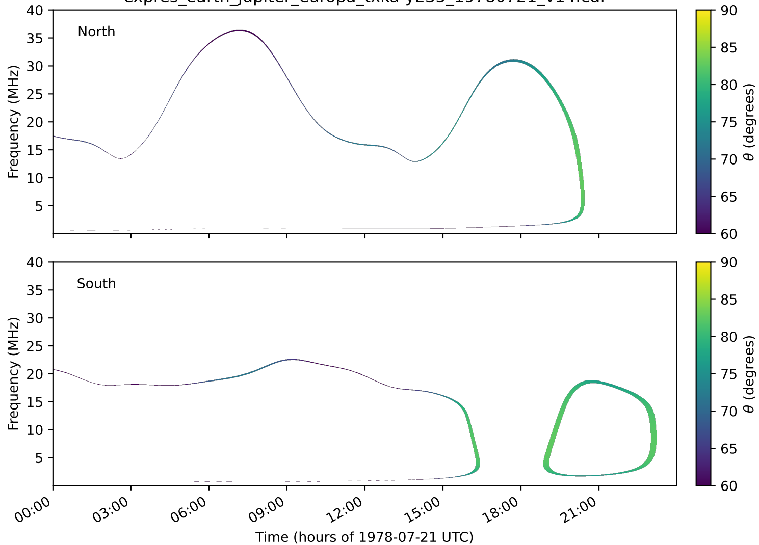
expres_earth_jupiter_europa_txka-y235_19780721_v14.cdf
