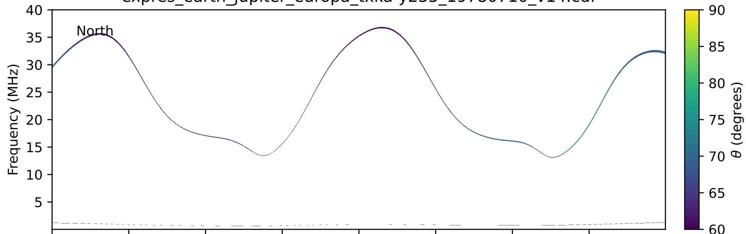
expres_earth_jupiter_europa_txka-y235_19780710_v14.cdf
