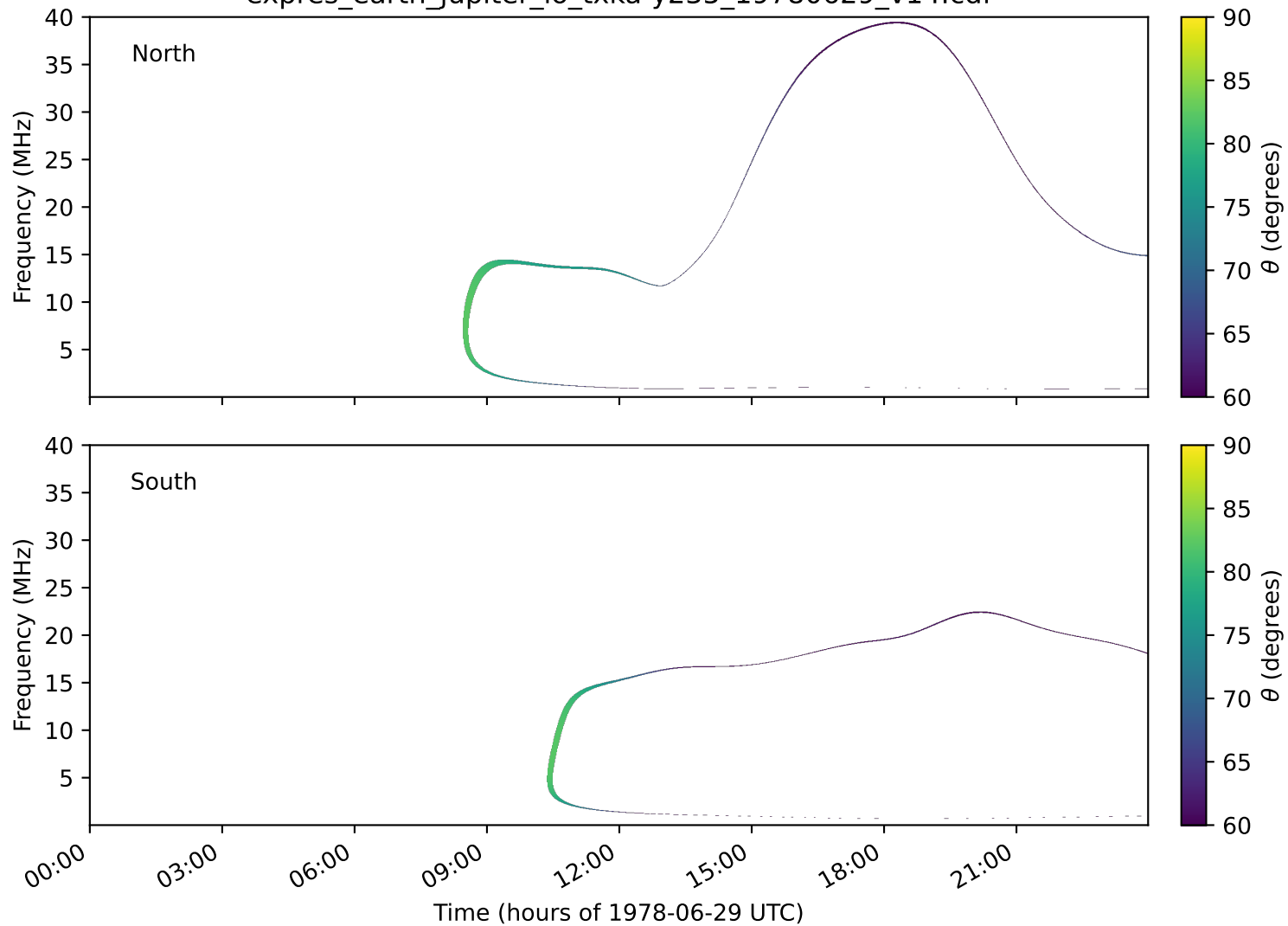
expres_earth_jupiter_io_txka-y235_19780629_v14.cdf
