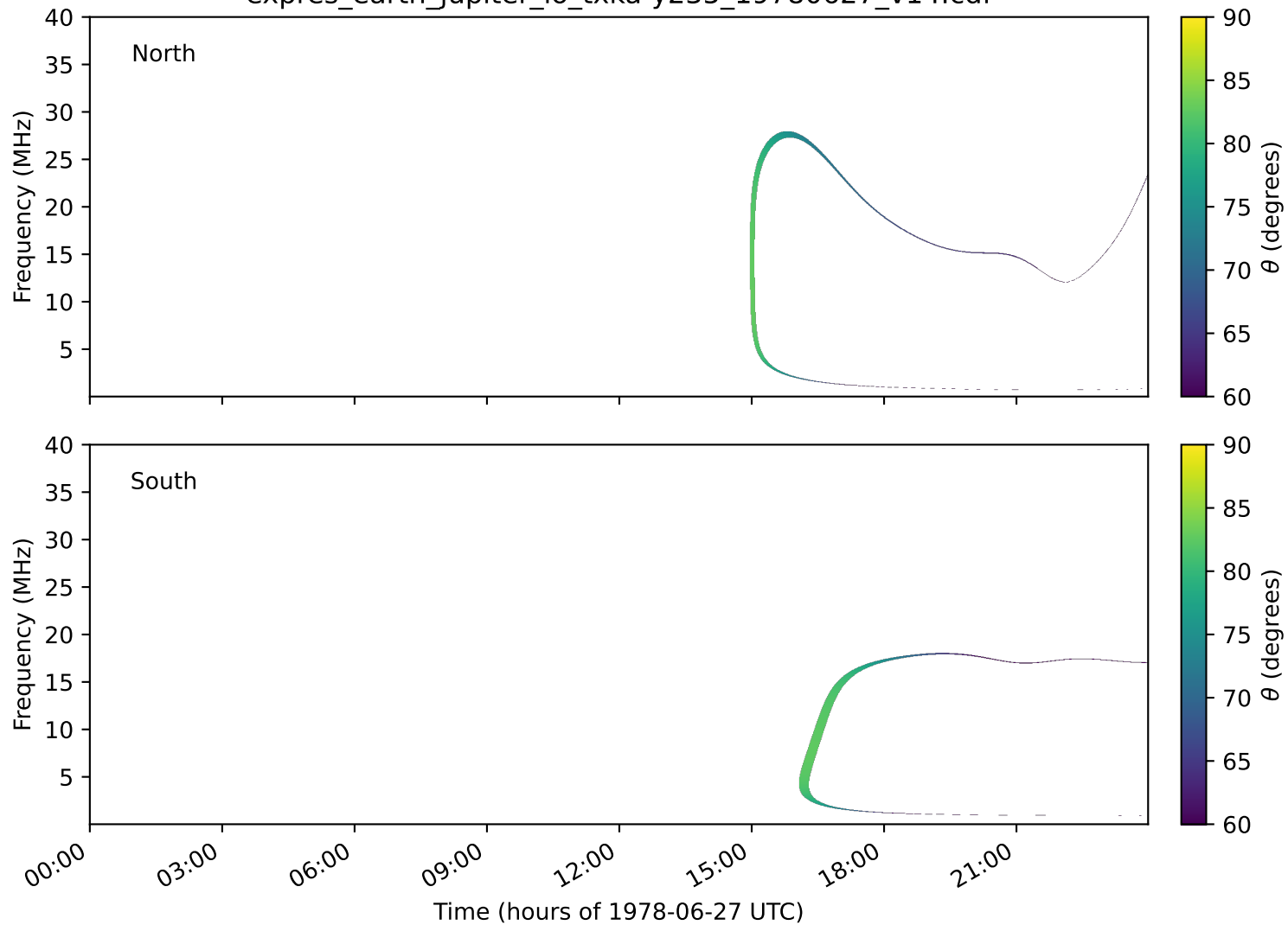
expres_earth_jupiter_io_txka-y235_19780627_v14.cdf
