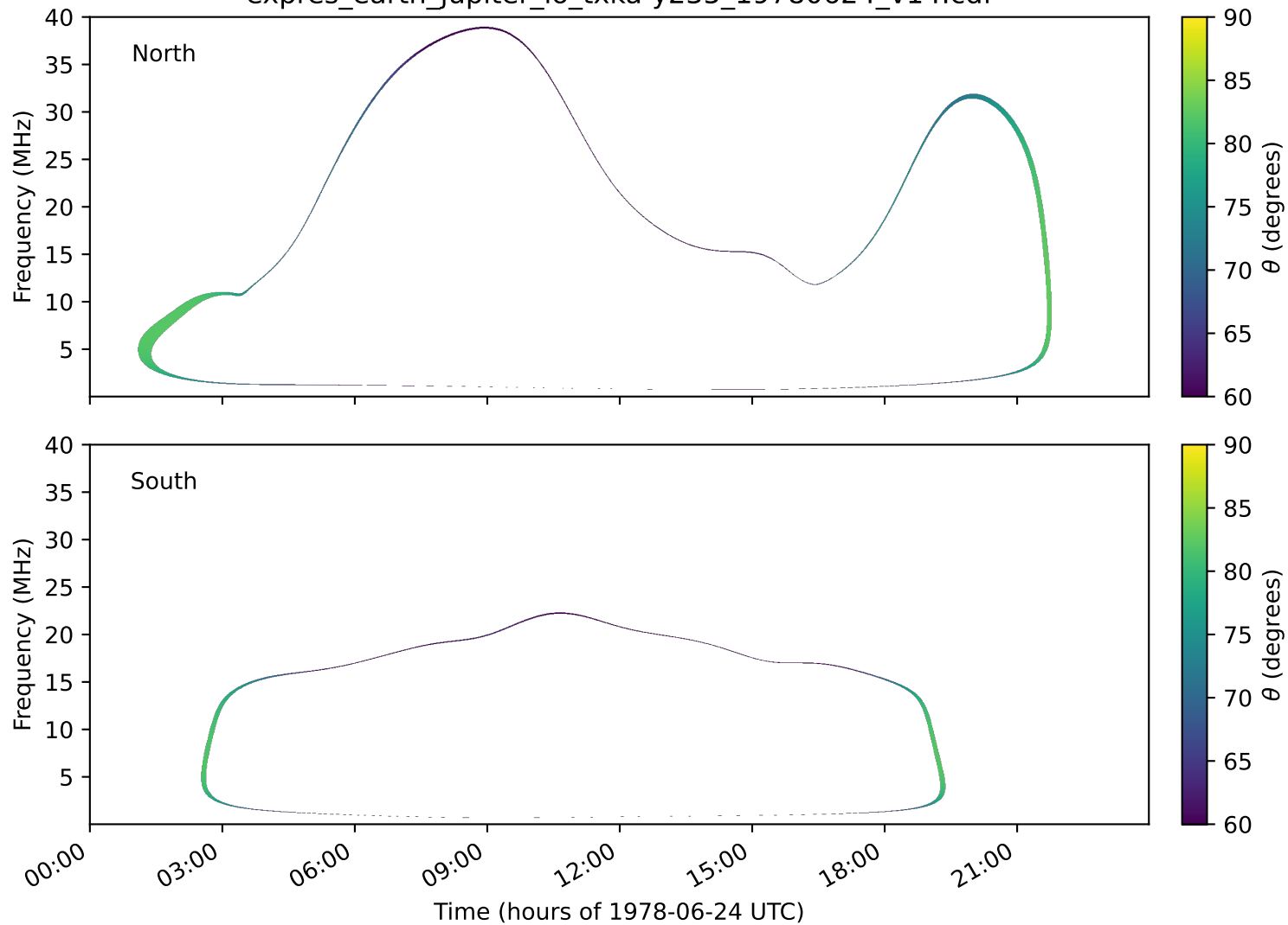
expres_earth_jupiter_io_txka-y235_19780624_v14.cdf
