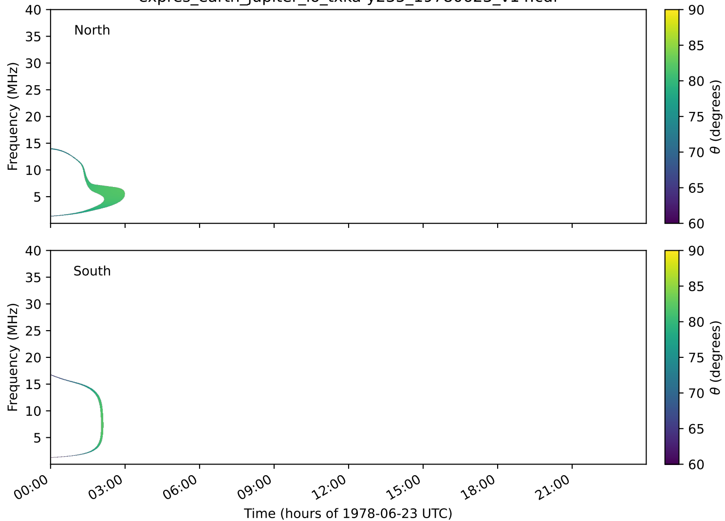
expres_earth_jupiter_io_txka-y235_19780623_v14.cdf
