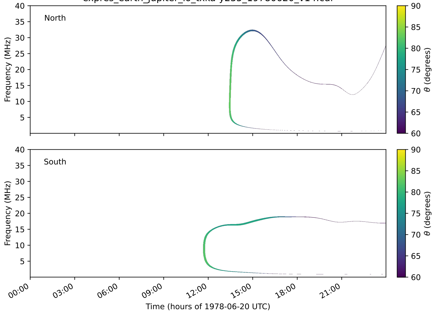
expres_earth_jupiter_io_txka-y235_19780620_v14.cdf
