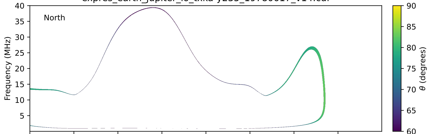
expres_earth_jupiter_io_txka-y235_19780617_v14.cdf
