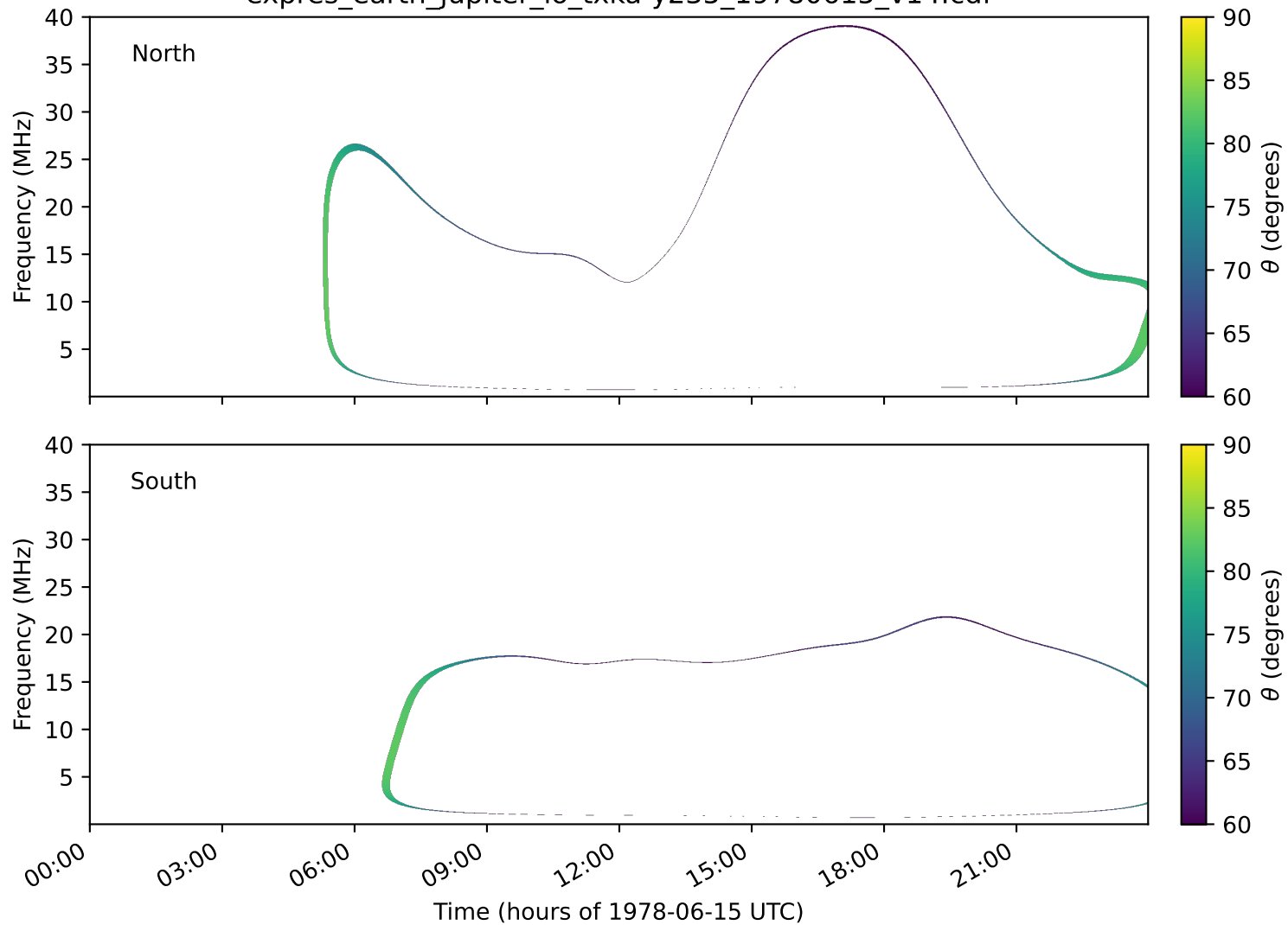
expres_earth_jupiter_io_txka-y235_19780615_v14.cdf
