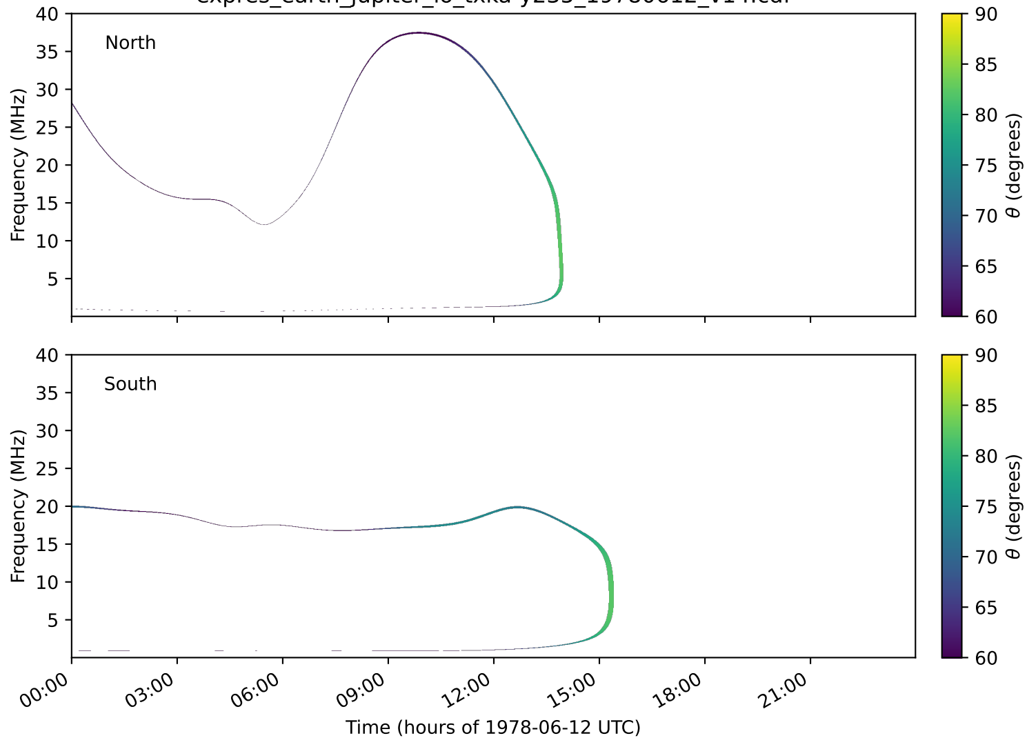
expres_earth_jupiter_io_txka-y235_19780612_v14.cdf
