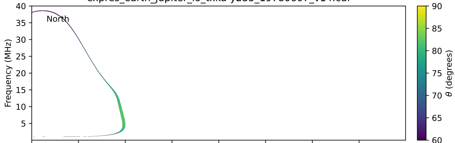
expres_earth_jupiter_io_txka-y235_19780607_v14.cdf
