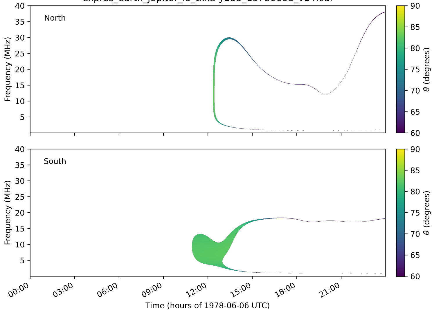
expres_earth_jupiter_io_txka-y235_19780606_v14.cdf
