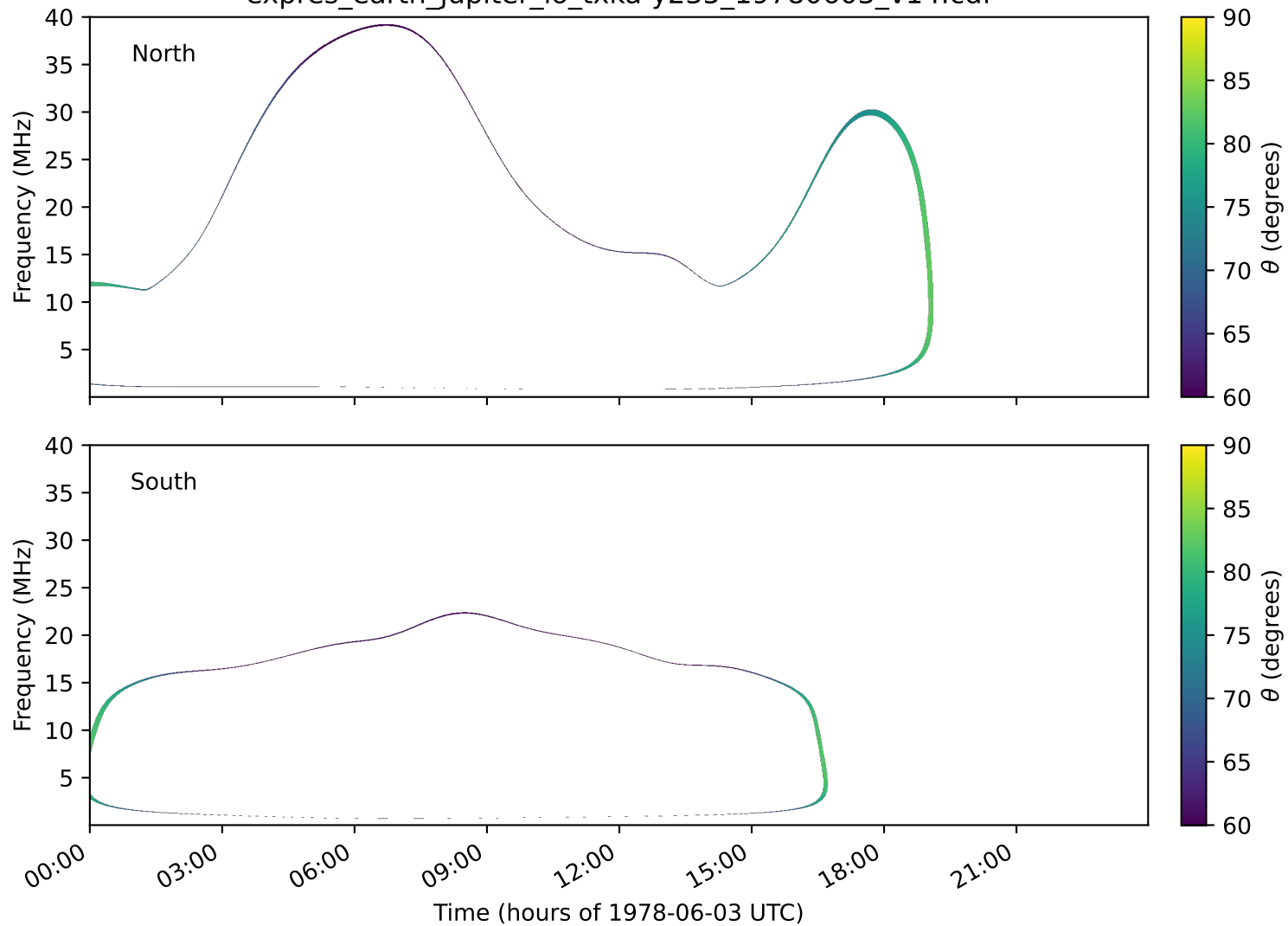
expres_earth_jupiter_io_txka-y235_19780603_v14.cdf
