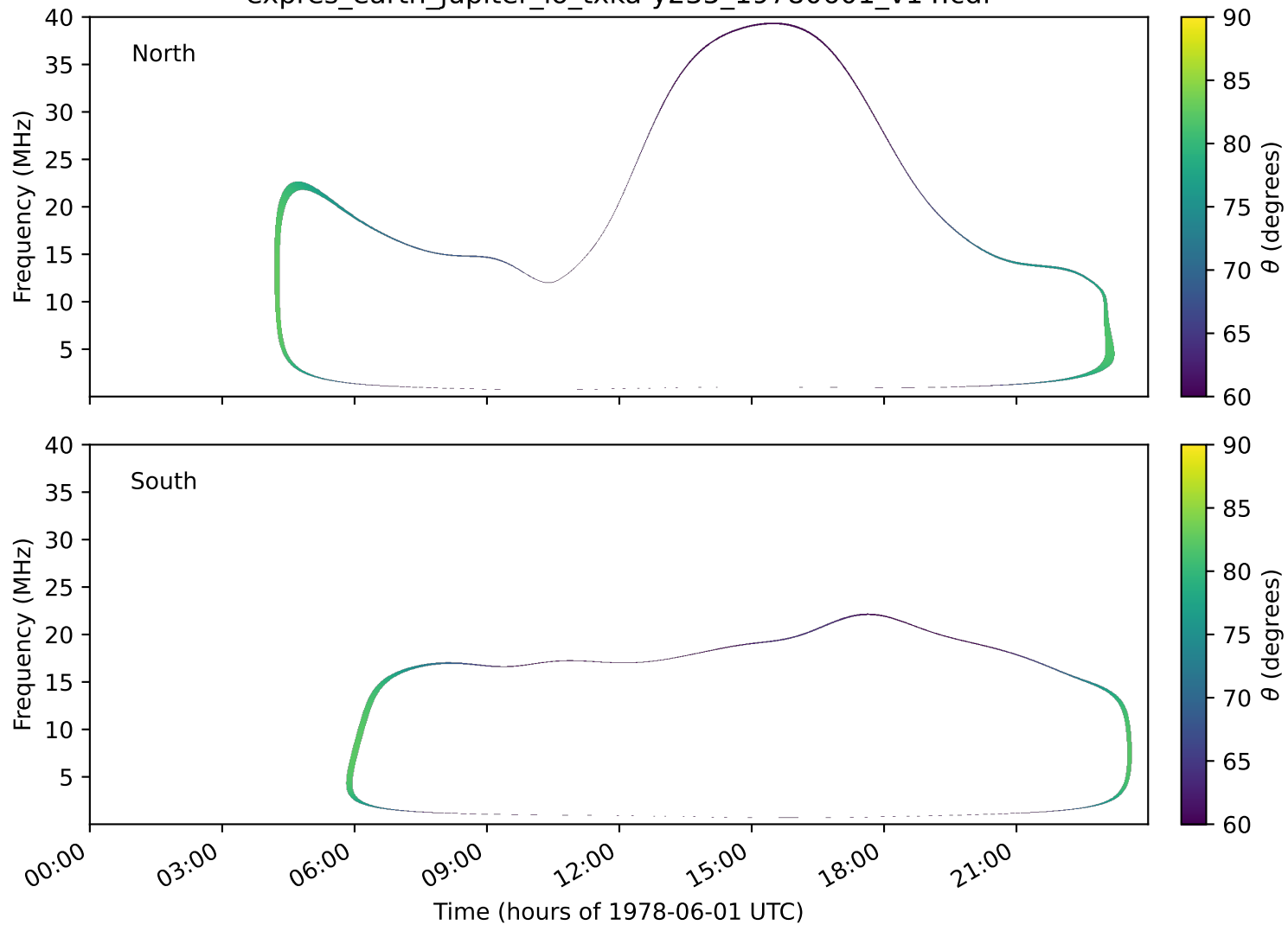
expres_earth_jupiter_io_txka-y235_19780601_v14.cdf
